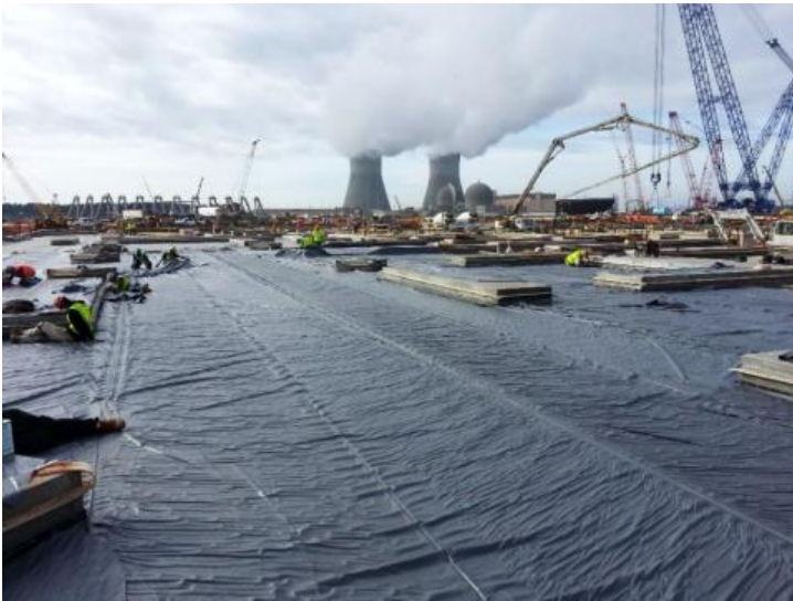
COOLING TOWER FOUNDATION LINER - 340,000 SF of PVC containment liner installed by USF.
